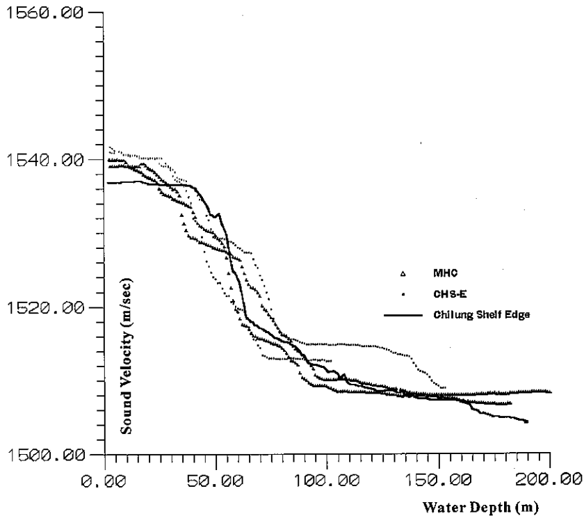
Fig. 9. Comparison plots among the acoustic profiles that situated in the Chilung Shelf and the Mien-Hua Canyon regions. The curved connected line denotes the acoustic profile in the location almost at the edge of the Chilung Shelf (Its location name denoted as Edge in Fig. 1). Small dots' profiles make the CHS-E type of acoustic profile shown in Fig. 10a.
