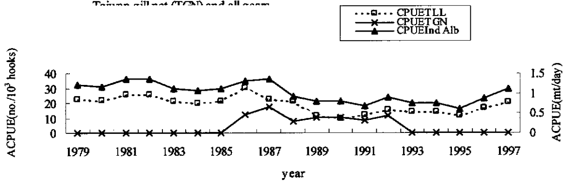
Fig. 2 The relative ACPUE series of albacore in the Indian Ocean calculated from the
