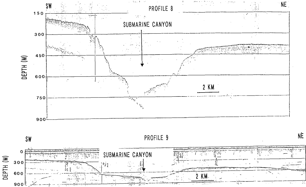
Fig. 10. Cross-sectional morphology of the segments of uppercanyon which is characterized by V-shaped configuration and high and steep walls. Location of the profile is shown in Figure 4.
