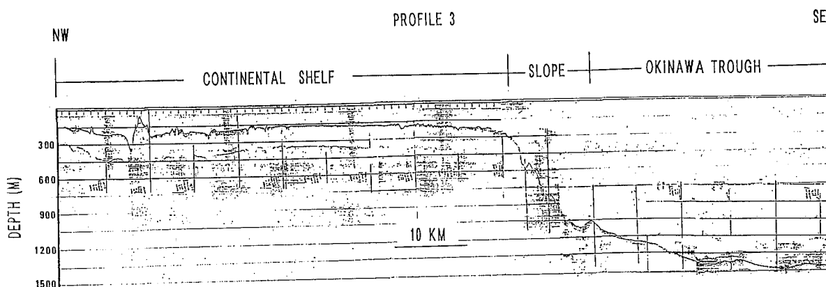
Fig. 11. Profile 3 trending NW/SE shows that the relatively flat continental shelf with locally low-relief features crosses the narrow and steep slope and extends onto the deep Okinawa Trough. Location of profile 3 is shown in Figure 4.
