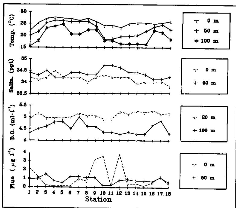
Fig. 2. Station specified line graph indicating water temperature (0, -50, -100 m); salinity (0, -50 m); dissolved oxygen (-20, -100 m); and fluorescence (0, -50 m).
