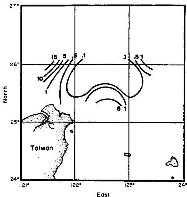
Fig. 4. Isopleth diagram of the biomass of fish eggs (g/1,000 m 3 ).
