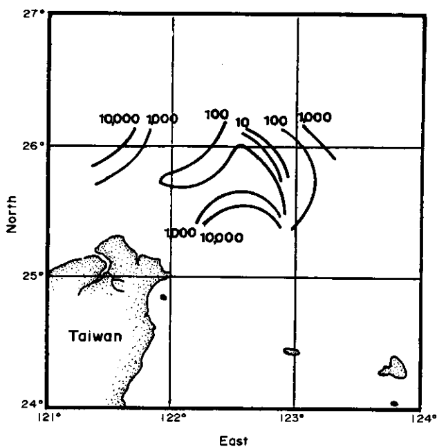
Fig. 3. Isopleth diagram of the counts of fish eggs (eggs/1,000 m 3 ).
