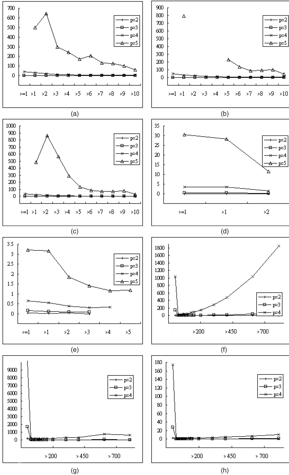
Fig. 2. Time-complexity charts with regard to choices of “ \sim d ” (Data collected with option EDGF). The Y-axis is with “time in second,” while the X-axis is with “ \sim d ” used in “ZC \sim d .” (a) TD(Linear). (b) TD(Lattice). (c) TD(Tree). (d) Leader-election. (e) PATHOS. (f) CSMA/CD(A). (g) CSMA/CD(B). (h) CSMA/CD(C).
