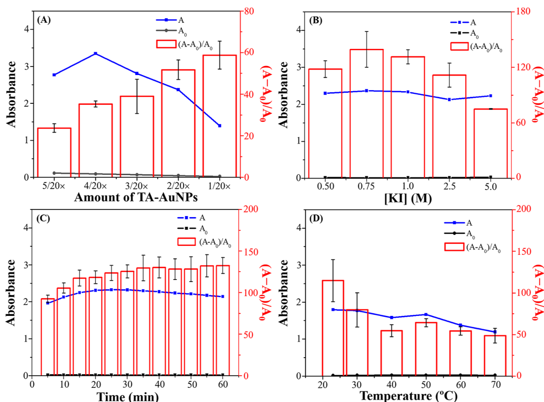
Figure 3. Determination of optimal conditions for \text{H}_2\text{O}_2 detection using the TA-AuNPs-3/ \text{I}^- system, analyzing variables: (A) TA-AuNPs-3 concentration, (B) KI concentration, (C) reaction time, and (D) assay temperature.
