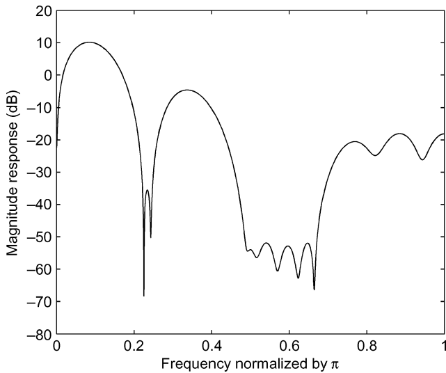
Fig. 6. The magnitude response of the TEQ.
