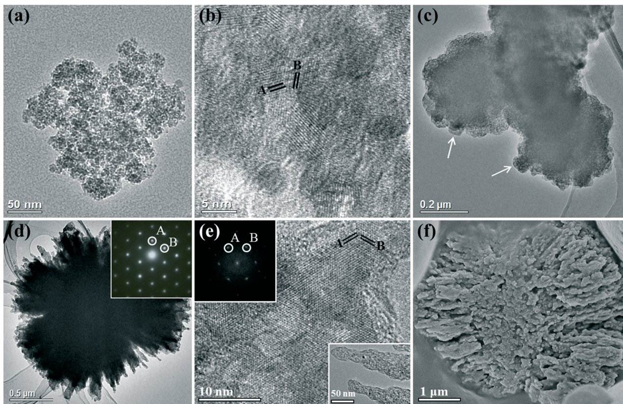
Fig. 3 SEM/TEM images of the vaterite phase from the 6 h specimen ( 28 \text{ g L}^{-1} gelatin, 2.86 \text{ M} urea). (a) TEM image of an aggregate of 5 \text{ nm} sized crystallites. (b) HRTEM image of a selected area in (a) showing vaterite nanocrystallites embedded in disordered precursor/gelatin molecules. The crystal fringes marked A and B can be indexed to the (101) and (100) planes of vaterite, respectively. (c) TEM image of clusters of weakly crystalline nanoparticles ( 50 \text{ nm} in diameter) as indicated by the arrows. (d) TEM image of a ball of needles particle produced by self-orientated attachment of nanoparticles. The inset is a corresponding SAED pattern recorded from a large area covering many needles. (e) HRTEM image taken at the edge of a spherulite particle showing a single crystalline-like domain structure with marked fringes indexed to A (100) and B (010) planes of vaterite. The upper inset is the corresponding FFT pattern. The lower inset is a low magnification TEM image of individual needles found at the edge of a spherulite particle. (f) SEM image of a broken ball of needles, showing the core area contains no needle morphology.
