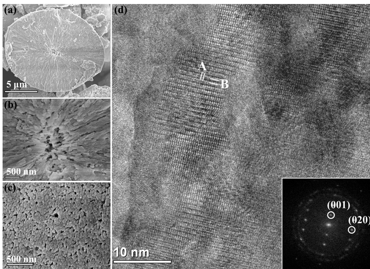
Fig. 4 SEM/TEM images of the vaterite phase from the 3 h specimen ( 28\ \text{g L}^{-1} gelatin, 5.71\ \text{M} urea). (a) Low magnification SEM image of a broken ellipsoid particle similar to that in Fig. 2b where the inner structure consists of densely packed needles. (b) An enlarged SEM image of the 1\ \mu\text{m} sized core region of the particle in (a) showing the core to be empty. (c) High magnification SEM image of the surface of an ellipsoid particle where needles, ca. \sim 40\ \text{nm} in diameter were found to radiate from the centre to the surface. (d) HRTEM image of a needle in an ellipsoidal particle (FFT pattern is shown inset) showing a domain structure with perfectly orientated fringes indexed to vaterite.
