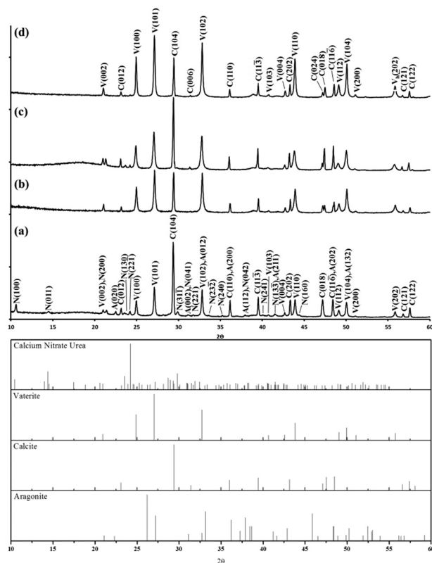
Fig. 1 PXRD patterns of specimens prepared using 28 g L -1 gelatin and 5.71 M urea with varying hydrothermal treatment times of, (a) 3 h, (b) 6 h, (c) 23 h, (d) 96 h. Pattern (a) is indexed to calcium nitrate urea (N), rhombohedral calcite (C), hexagonal vaterite (V) and orthorhombic aragonite (A) phases whilst pattern (d) is indexed to the rhombohedral calcite (C) and hexagonal vaterite (V) crystal structures, respectively.
