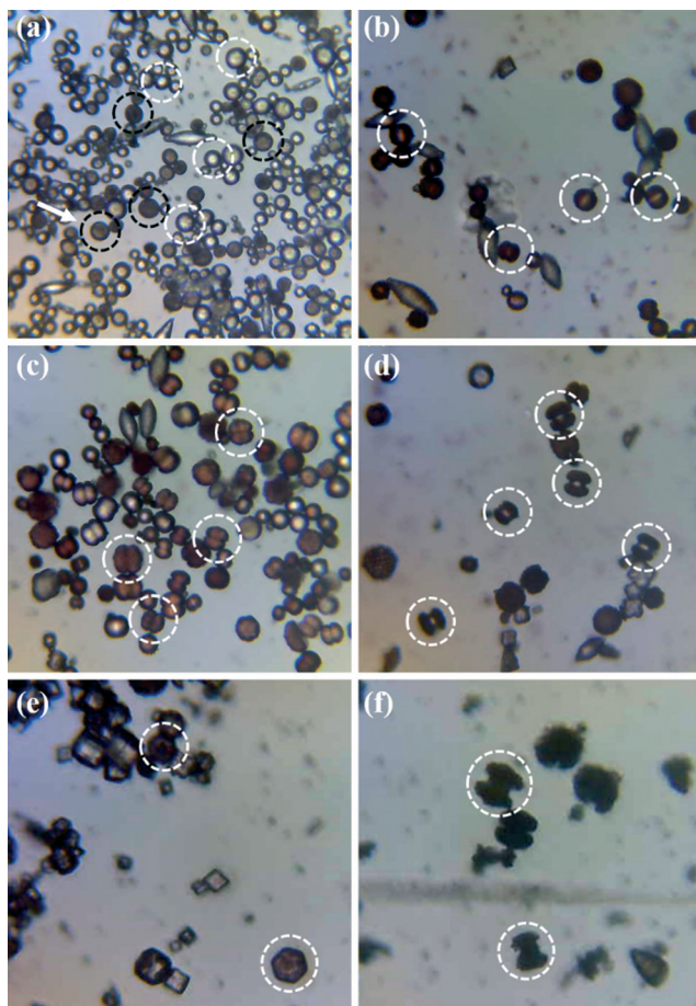
Fig. 8 Optical microscopic images of vaterite mesocrystals stained with cationic safranin T dye. Growth stages include (a) ellipsoid, (b) embryonic, (c) twin-cauliflower, (d) dumbbell, and (e) hexagonal prism particles. (f) Dumbbell particles calcined at 600 °C for 4 h prior to the addition of safranin T dye. The black ring outside all mesocrystals is not dye molecules but fringes formed from the interference between light rays reflected from the surface of the mesocrystal.
