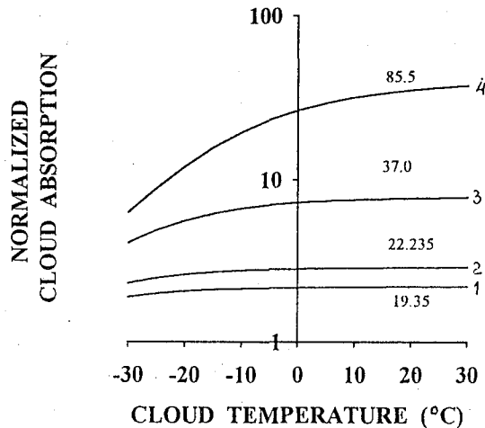
Fig. 9. The dependencies of cloud absorption at the SSM/I frequencies on cloud droplet temperature normalized relative to f_0 = 13.1 GHz: (1) f = 19.35 GHz, (2) f = 22.23 GHz, (3) f = 37.0 GHz, and (4) f = 85.5 GHz.
