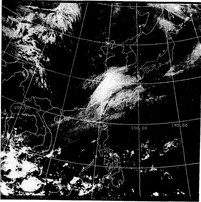
Fig. 6. The GMS-4 IR image taken at 0632 GMT (local standard time 14:32), March 19, 1994.
