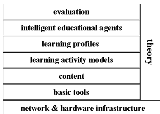
Fig. 11. Layered architecture of network learning.
