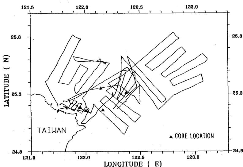
Fig. 2. Location of echo-sounding tracks, 3.5 kHz subbottom profiles and five box-cored samples. The surveys covered most of the areal extent of the Huapinghsu Channel/Canyon System.
