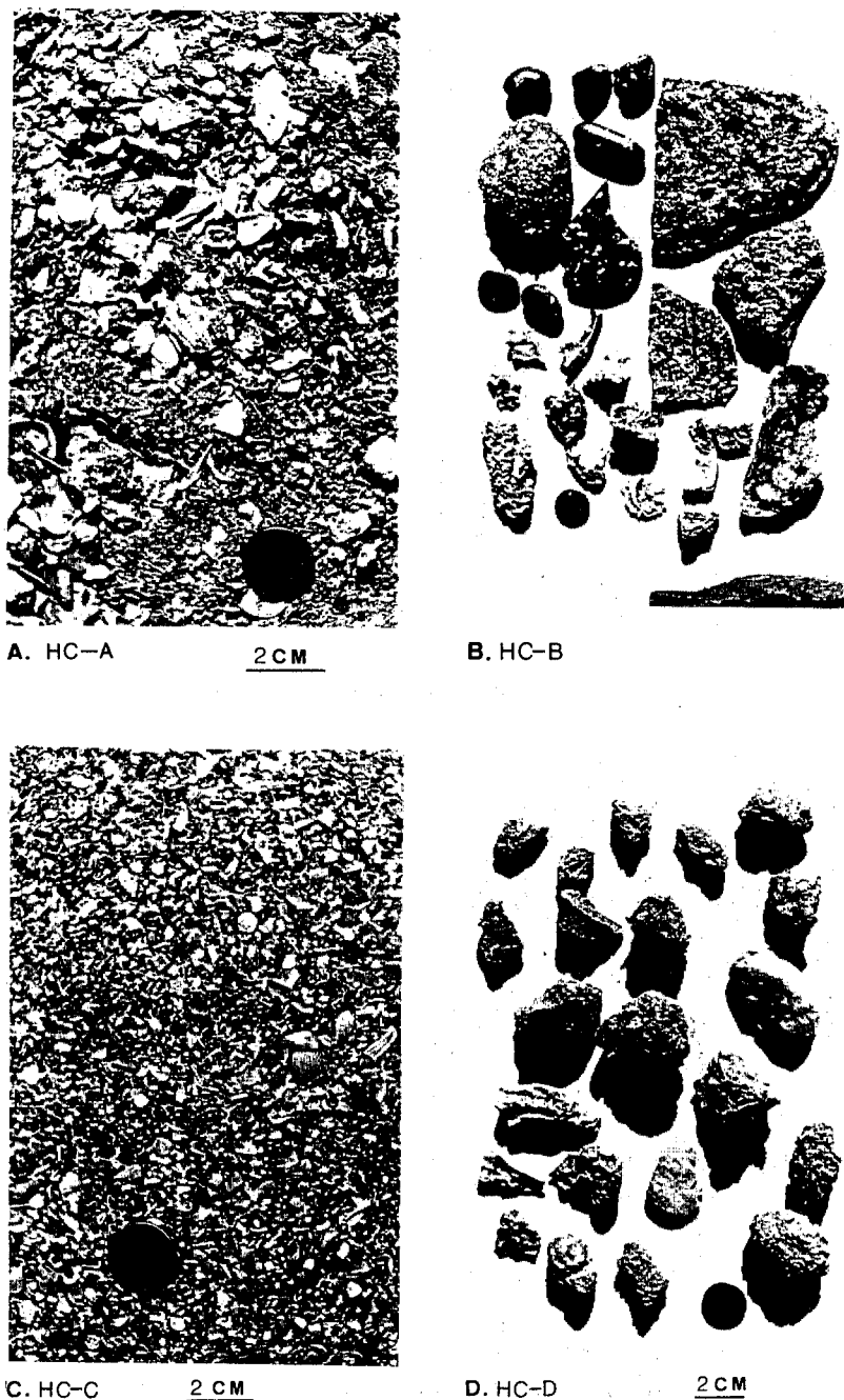
Fig. 7. Five box-cored samples indicate that coarse-grained sediments are the dominant surface sediments in the channel and adjacent shelves and muddy deposits occur around the canyon mouth and nearby slopes. (HC-A) and (HC-B) Pebbly sands and gravels, (HC-C) Coarse-grained shell fragments, (HC-D) Gravelly mudclasts and rock fragments and (HC-E) Fine-grained silts and clays. Locations of the cores are shown in Fig. 3.
