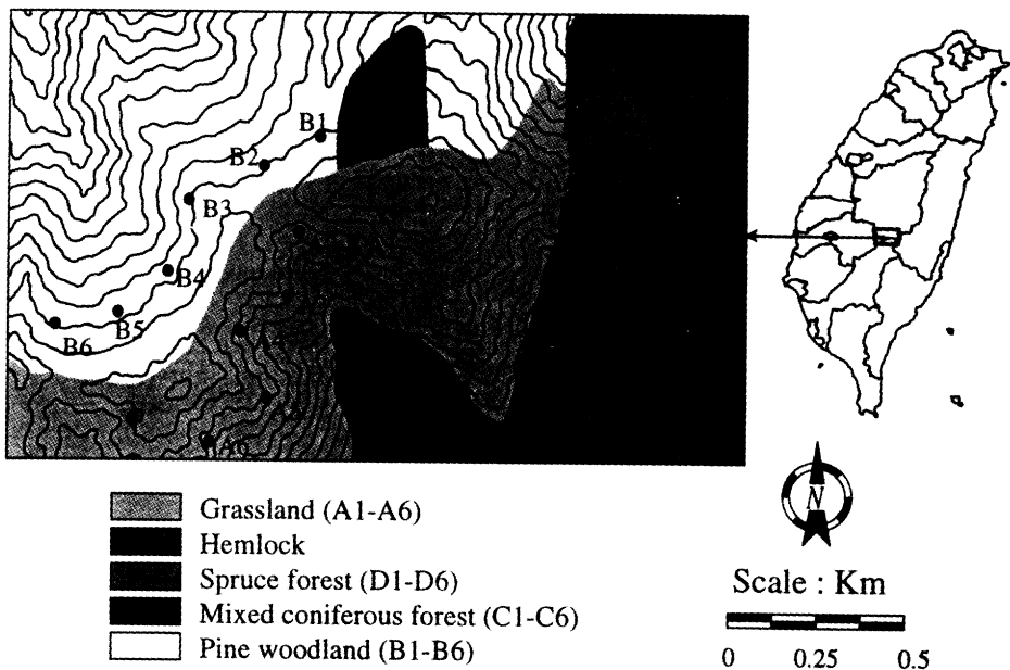
Figure 1 A location map of the bird sampling points in four plant communities at Tatachia, Yushan National Park, Taiwan.
