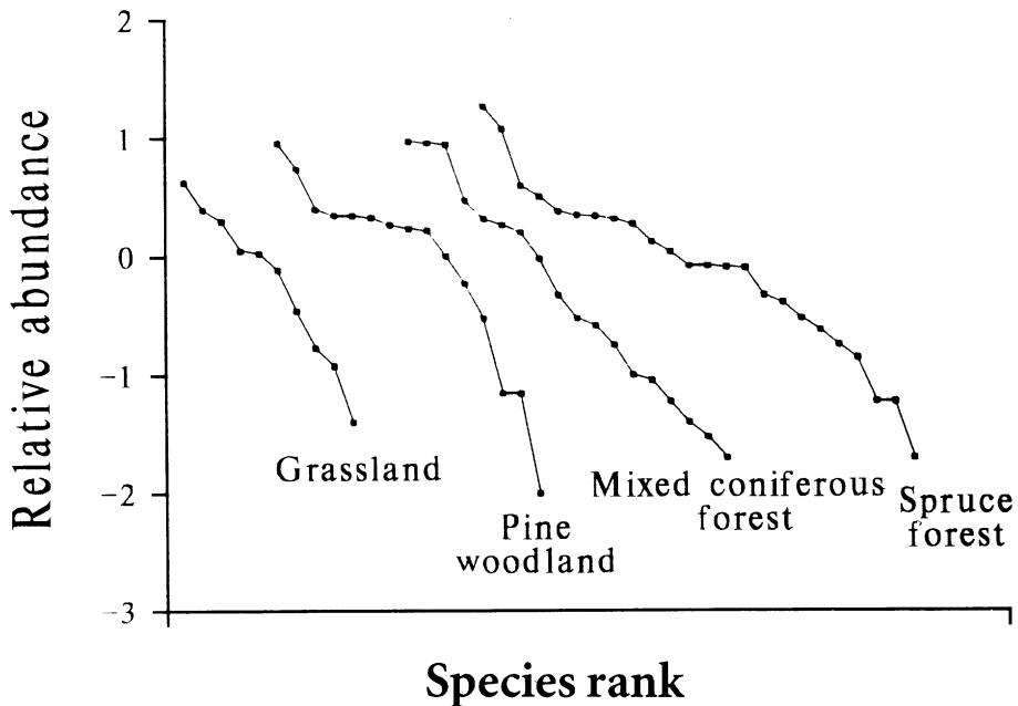
Figure 2 Species rank curve for the four avian communities in the Tatachia area of Yushan National Park, central Taiwan. The curve for the grassland bird community is close to a geometric curve and the curve for the spruce forest bird community is close to a log-normal distribution. The others fall between these two extremes.
