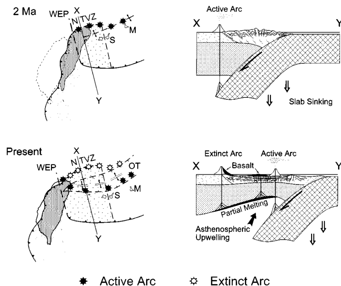
Figure 1. Tectonic evolution of northern Taiwan volcanic zone (NTVZ). Left is the plane views, and right is the corresponding cross sections. Note that arc volcanism was active in NTVZ at 2 Ma but later migrated to the Okinawa Trough. Asthenospheric upwelling induced by lithospheric stretching may trigger partial melting of the decompressed mantle to yield magmas of ocean-island-basalt signature. WEP—western edge of subducting Philippine Sea plate, S—Ishigakijima, M—Miyako-jima, OT—Okinawa Trough (modified from Fig. 4 of Teng, 1996).
