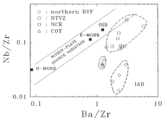
Figure 1. Nb/Zr versus Ba/Zr diagram. Abbreviations are as follows: NTVZ—the northern Taiwan volcanic zone, COT—the central Okinawa Trough, RVF—the Ryukyu volcanic front, IAB—ocean island basalt, NCK—the northwestern and central Kyushu, OIB—ocean island basalt, MORB—mid-ocean-ridge basalt. The data of the COT and the NCK as well as the NTVZ are from Ishizuka et al. (1990) and Chen et al. (1996), respectively. The values of OIB, E-MORB, and N-MORB are from Sun and McDonough (1989).
