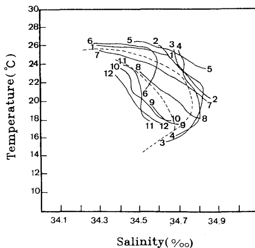
Fig. 2. The selected T-S lines from station groups of A, B, and C.
