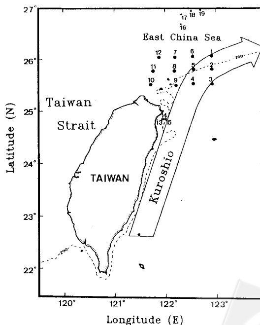
Fig. 1. Sampling stations and station groups in the ichthyoplankton study in the Kuroshio edge area and the adjacent waters.
