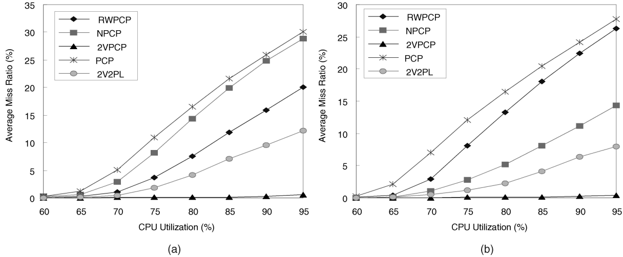
Fig. 17. The miss ratios of (a) server-side transactions and (b) client-side (read-only) transactions: one server, one client, database size was 50.
