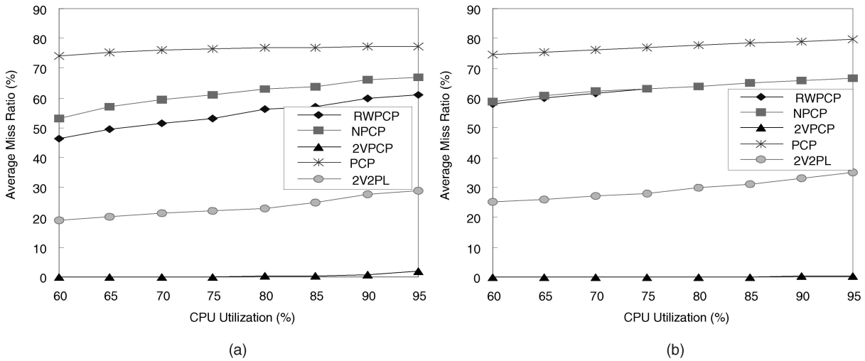
Fig. 15. The miss ratios of (a) server-side transactions and (b) client-side (read-only) transactions: one server, 10 clients, database size was 50.
