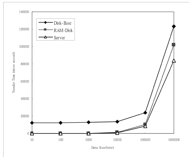
Fig. 6. Data access time plus memory-copying time for databases of various sizes: No log processing time is included.
