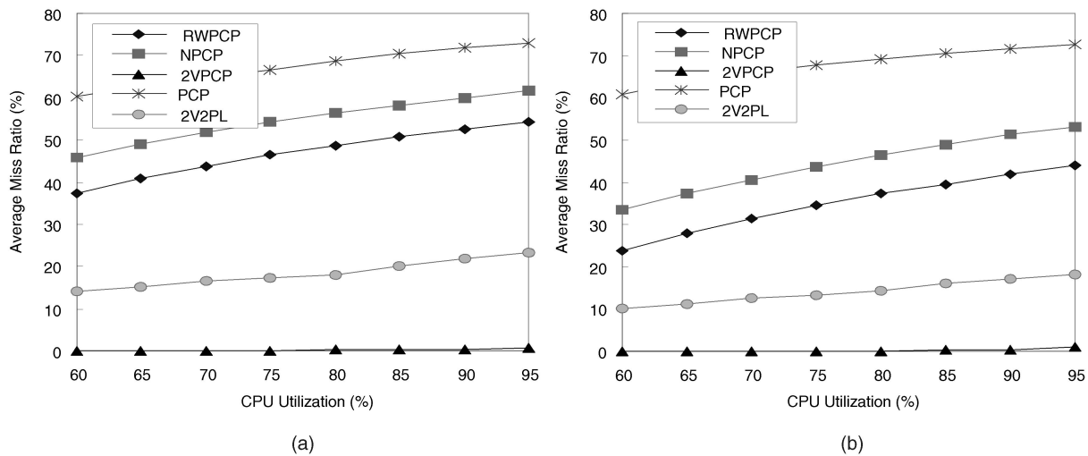
Fig. 12. The miss ratio of server-side transactions: one server, five clients, database size was (a) 50 or (b) 100.
