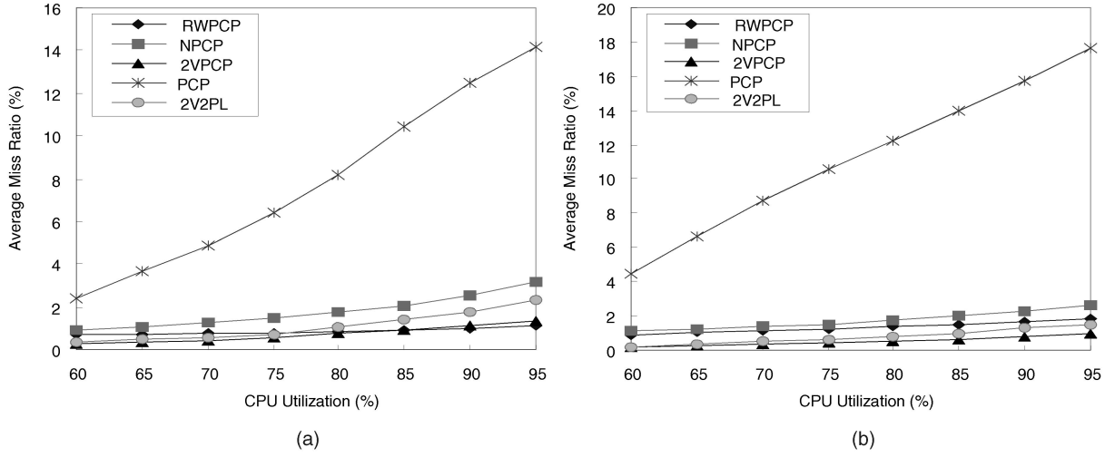
Fig. 14. The miss ratio of the top one fourth highest-priority server-side transactions: one server, five clients, database size was (a) 50 or (b) 100.
