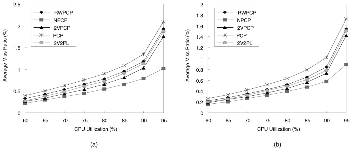
Fig. 7. The miss ratio of all transactions: single processor, database size was (a) 15 or (b) 25.
