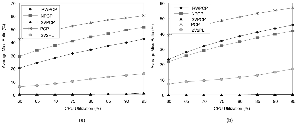
Fig. 16. The miss ratios of (a) server-side transactions and (b) client-side (read-only) transactions: one server, three clients, database size was 50.
