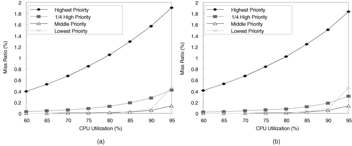
Fig. 19. The miss ratio of the client-side transactions: one server, five clients, database size was (a) 50 or (b) 100, the updating transaction \tau_{Upd} had the highest, top one fourth, middle, or lowest priority in the system.
