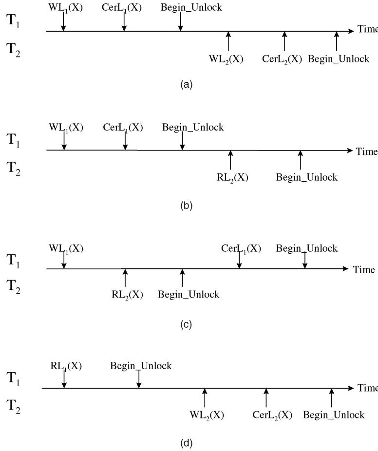
Fig. 4. Serializability order of conflicting transactions. (a) W/W conflict. (b) W/R conflict: W proceeds R. (c) W/R conflict: R proceeds W. (d) R/W conflict.
