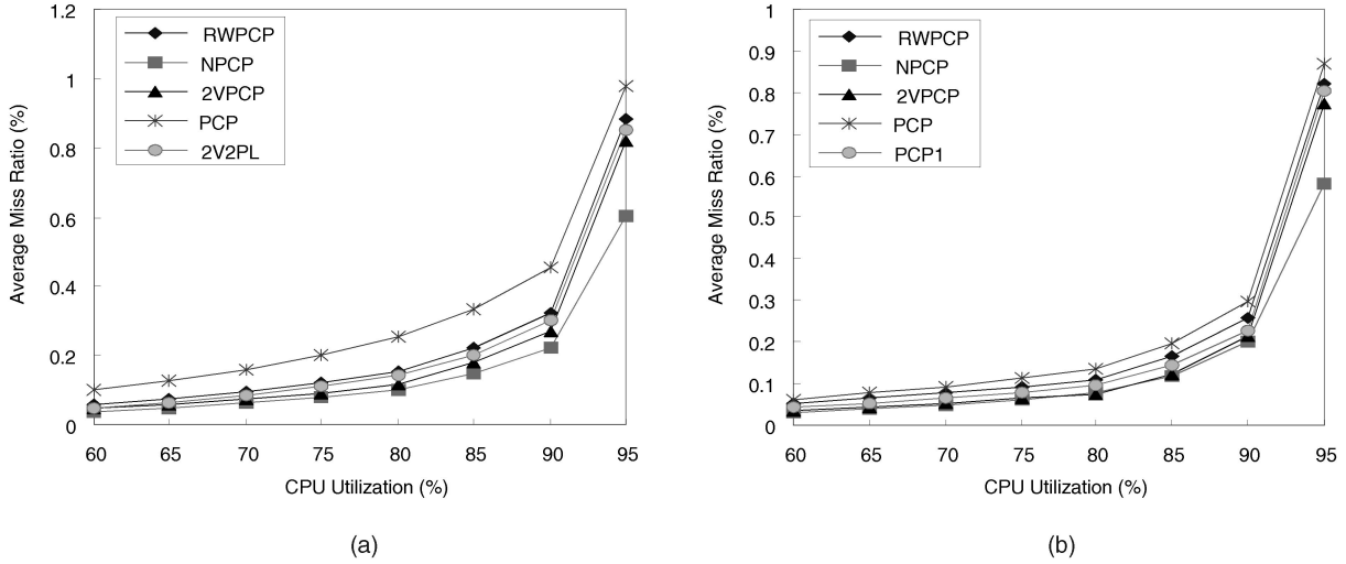
Fig. 9. The miss ratio of all transactions: single processor, database size was (a) 150 or (b) 200.
