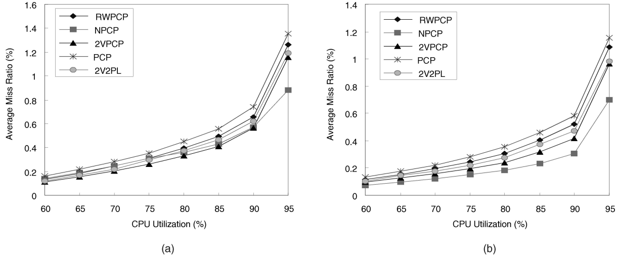
Fig. 8. The miss ratio of all transactions: single processor, database size was (a) 50 or (b) 100.
