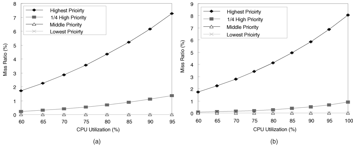
Fig. 18. The miss ratio of the top one fourth highest-priority client-side transactions: one server, five clients, database size is (a) 50 or (b) 100, the updating transaction \tau_{Upd} had the highest, top one fourth, middle, or lowest priority in the system.
