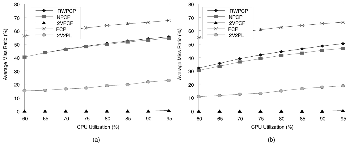
Fig. 13. The miss ratio of client-side (read-only) transactions: one server, five clients, database size was (a) 50 or (b) 100.
