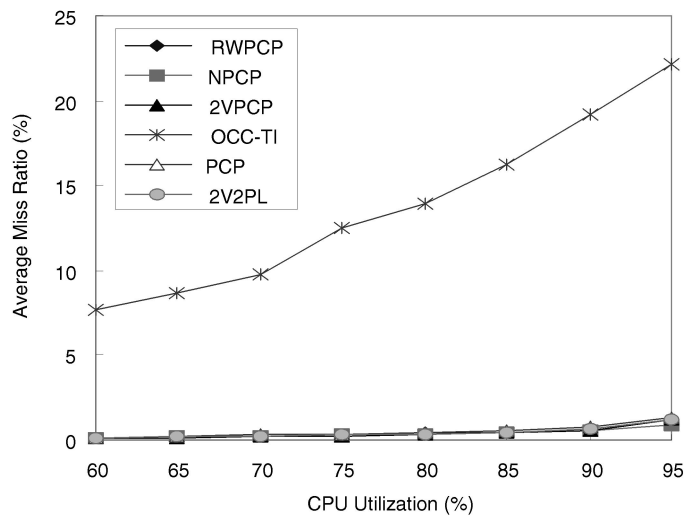
Fig. 11. The miss ratio of all transactions scheduled by optimistic concurrency control protocol, PCP, RWPCP, NPCP, 2V2PL, and 2VPCP when the database size was 50.
