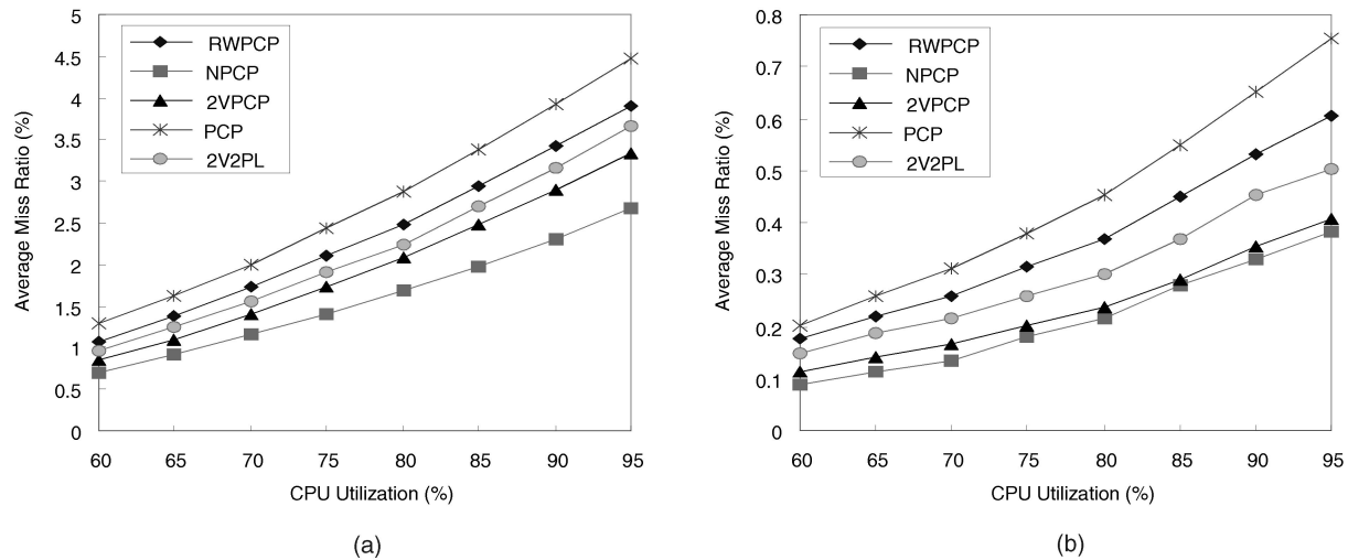
Fig. 10. The miss ratio of the top one fourth highest-priority transactions: single processor, database size was (a) 15 or (b) 200.
