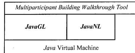
Figure 12. The system hierarchy of a multi-participant building walkthrough application using JavaGL and JavaNL.
