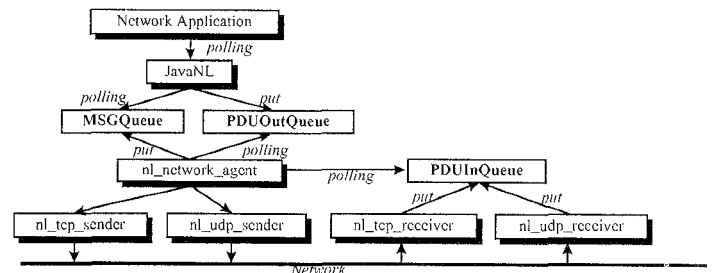
Figure 7 PDU sending and receiving in JavaNL.
